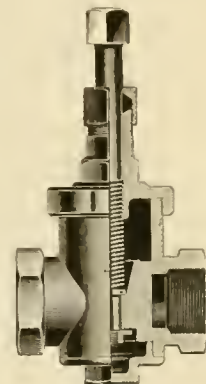
ASHTON BLOW-OFF VALVE.
